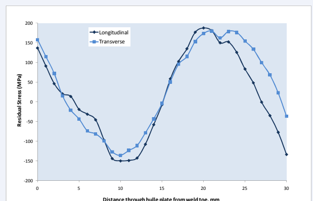
Fig. 5: Estimated residual stresses arising from bending the hull plate
