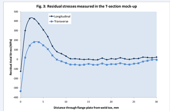
Fig. 3: Residual stresses measured in the T-section mock-up
