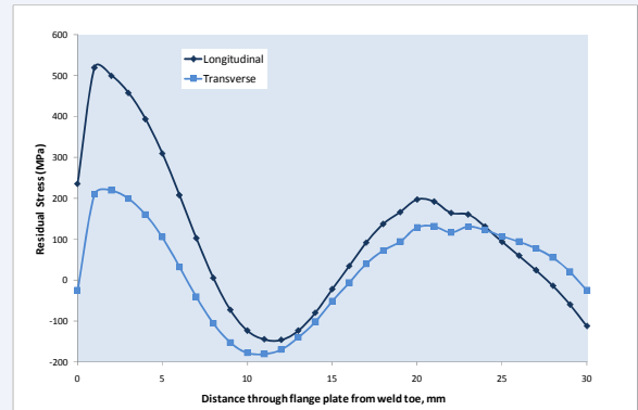
Fig. 4: Residual stresses measured in the full-scale section
